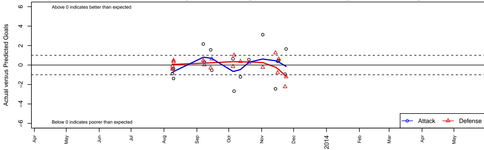
Peninsula SC Fury Blue B96 Dots are actual minus expected GF (blue circles) and GA (red triangles). Blue line is smoothed change in attack strength. Red is smoothed change in defense strength.
